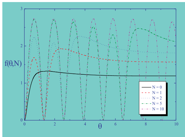
Figure 2: Absolute value squared of the two particle form factors f(\theta, N) = |\hat{F}_2^{\Theta}(\theta, N)|^2 / 2\pi^2 as functions of the rapidity for different values of N for \omega = 1.3 and x = 0.1 .
