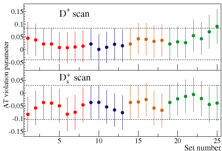
Fig. 6. T -violating asymmetry A_{T_{\text{viol}}} versus several sets of cuts. We varied the \sigma_L from 4 to 12 (8 points), Iso2 from 10^{-2} to 10^{-6} (5 points), confidence level of the secondary vertex from 1% to 5% (5 points), \Delta_K from 2 to 5 (7 points). The dashed lines show the quoted A_{T_{\text{viol}}} asymmetry \pm 1\sigma .
