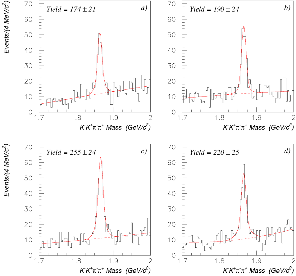
Fig. 2. K^- K^+ \pi^- \pi^+ invariant mass distributions for: (a) D^0 sample with C_T > 0 , (b) D^0 sample with C_T < 0 , (c) \bar{D}^0 sample with \bar{C}_T > 0 and (d) \bar{D}^0 sample with \bar{C}_T < 0 . The fit (solid curve) is explained in the text.
