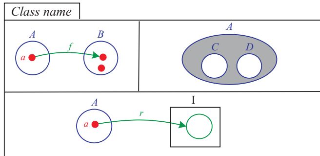
Figure 1: An invariant
