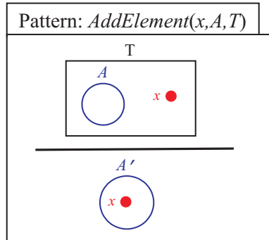
Figure 7: Add element
