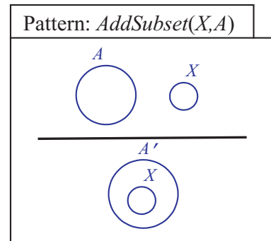
Figure 8: Add subset
