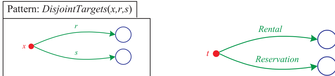
Figure 4: Disjoint targets
