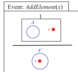
Figure 2: Event specification
