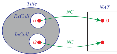
Figure 10: Combining patterns
