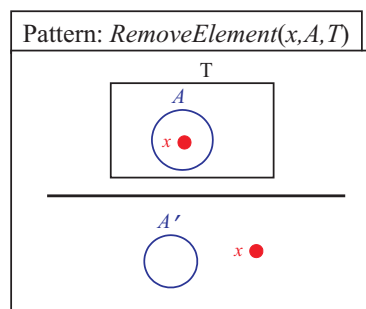
Figure 9: Remove element
