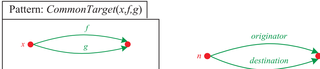
Figure 5: Common target
