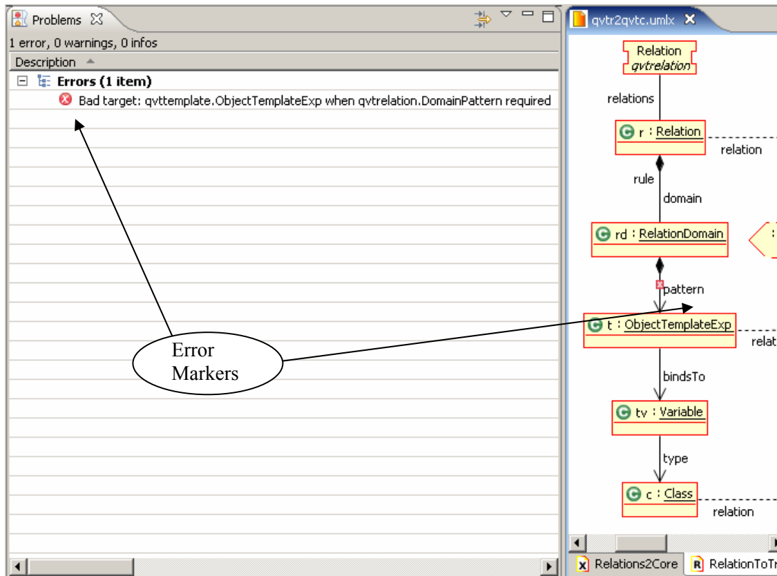
Figure 6 UMLX Views with errors
