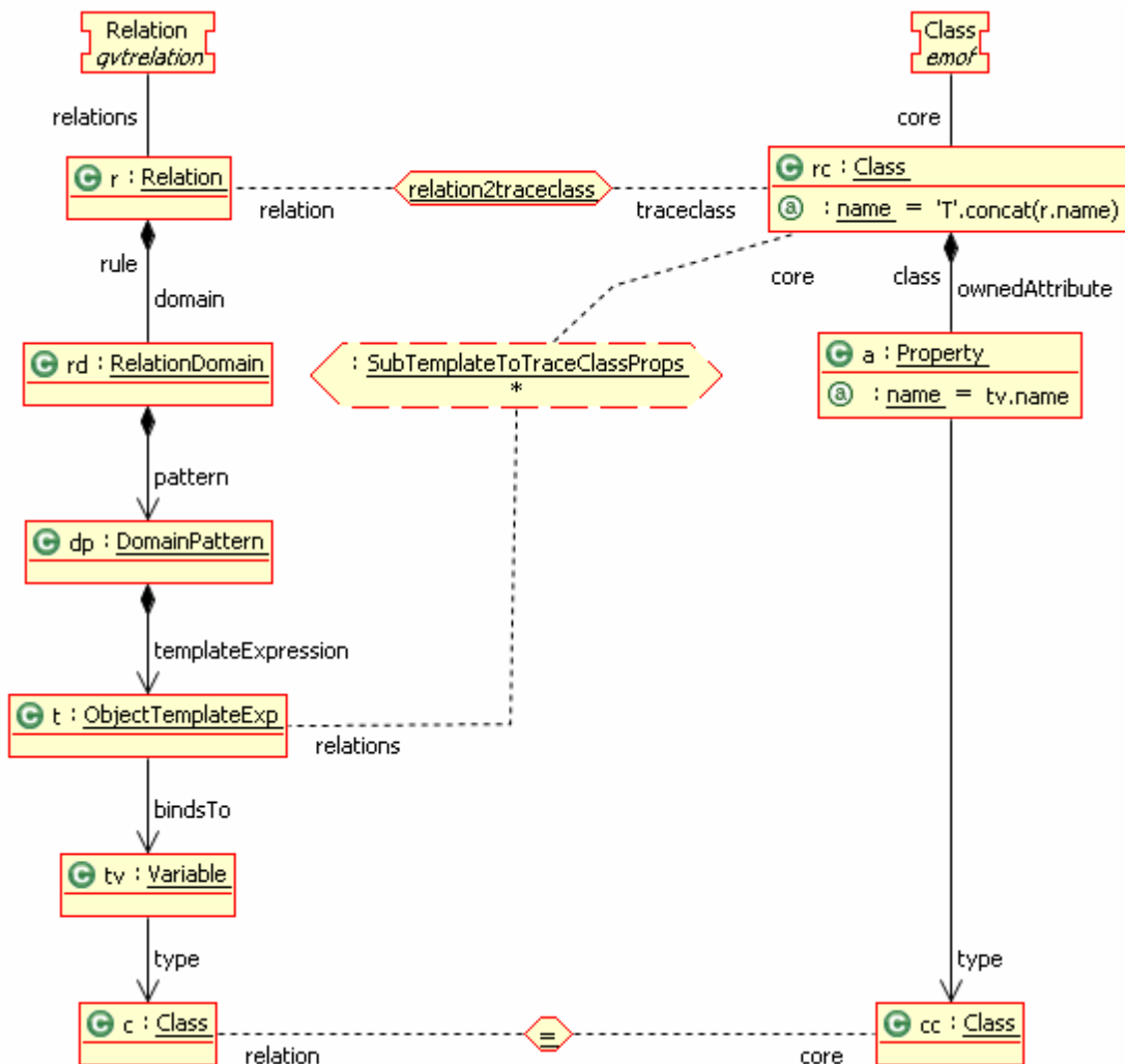
Figure 4 UMLX version of RelationToTraceclass Relation
