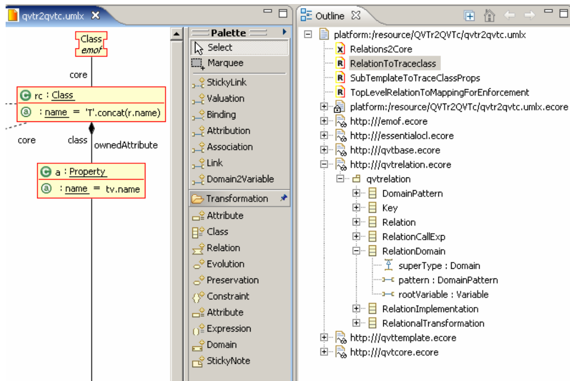
Figure 5 UMLX Palette and Outline
