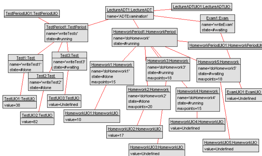
Fig. 4. A snapshot of the process instance with activities and corresponding UI objects
