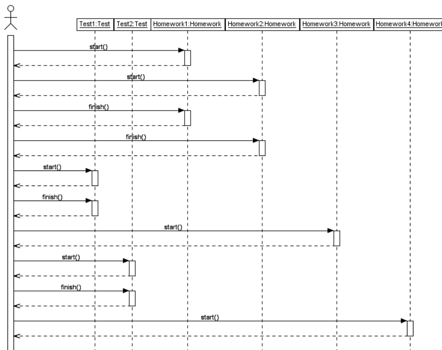
Fig. 5. A sequence diagram showing the scenario until the snapshot of Figure 4 is taken
