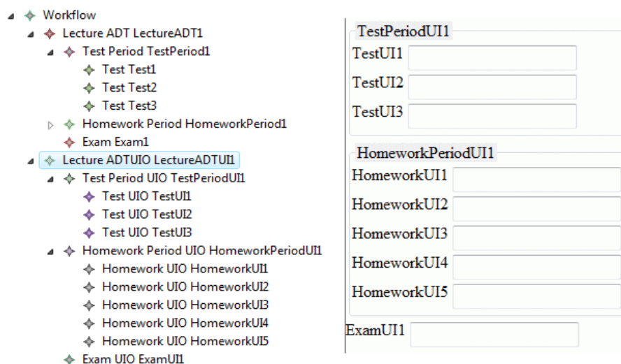
Fig. 8. Ecore model and generate user interface
