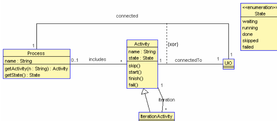
Fig. 1. The meta-model for the declarative business process modeling approach
