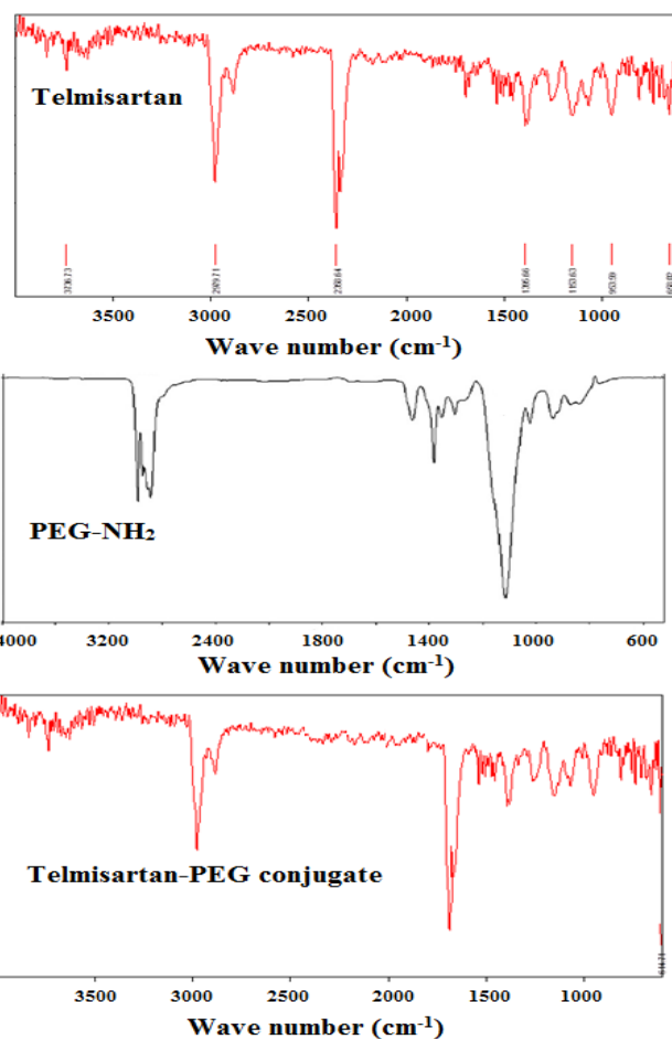
Figure 1: FT-IR spectrum of telmisartan, PEG-NH 2 and telmisartan-PEG conjugate.
