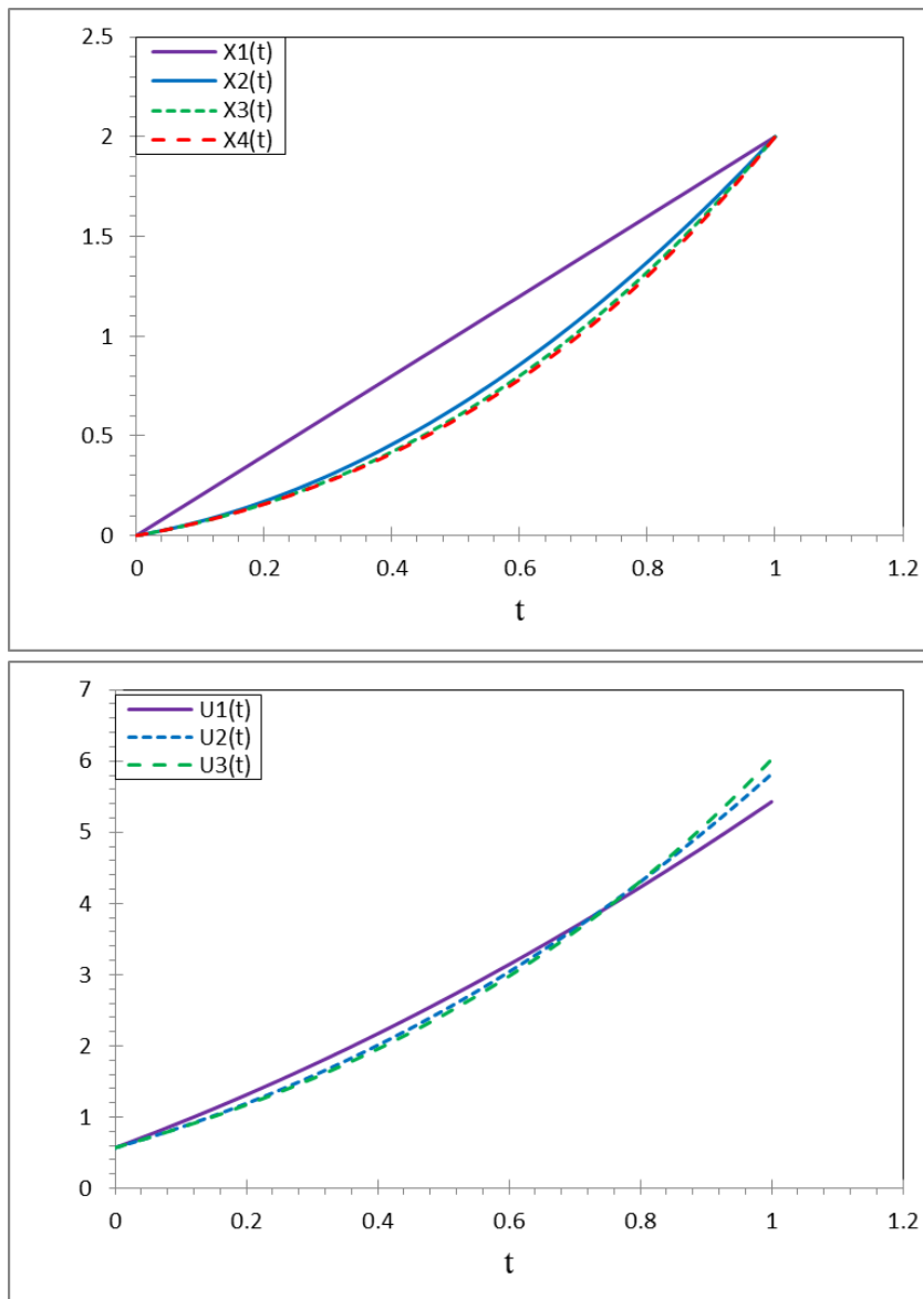
Fig. 2 Solution of Example 2. The solution of the first iterative compared with the exact solution.
