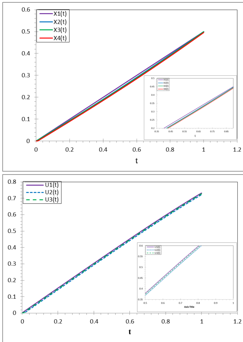
Fig. 3 Solution of Example 3. The solution of the first iterative compared with the exact analytical solution.
