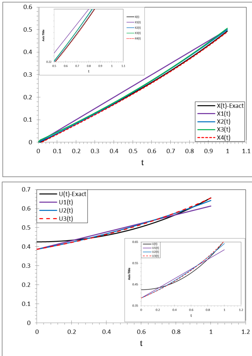
Fig. 4 Solution of Example 4. The solution of the first iterative compared with the exact solution.
