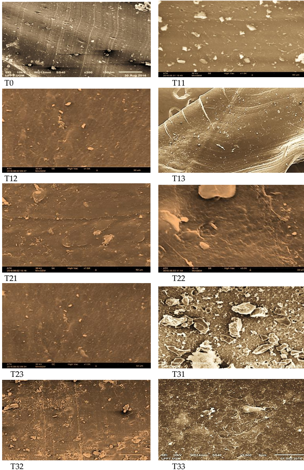
Figure 3. SEM of gelatin combination surfaces (Magnification 2000x). T0= gelatin bovine split hide; T11, T12, T13= gelatin bovine split hide : SPI = 90 : 10 + TG ase enzyme 10, 20, 30 U; T21, T22, T23= gelatin bovine split hide : SPI = 80 : 20 + TG ase enzyme 10, 20, 30 U; T31, T32, T33= gelatin bovine split hide : SPI = 70 : 30 + TG ase enzyme 10, 20, 30 U.
