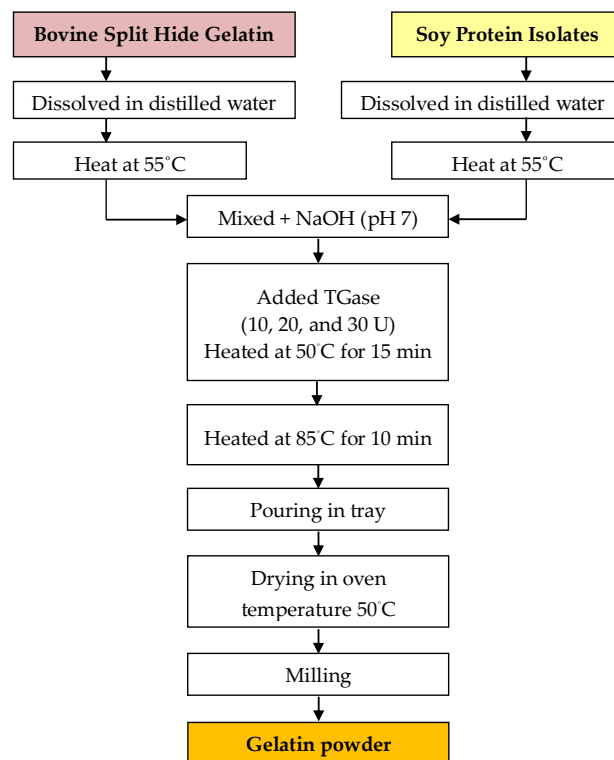
Figure 1. Flowchart of the manufacture of gelatin in combination with bovine split hide and soy protein isolate with the addition of the transglutaminase enzyme (Adapted from Chambi & Grosso, 2006).
