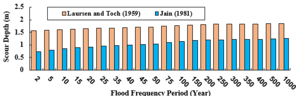
Fig. 11. Scour depth of the Simineh Road bridge piers using the equations between Larsen and Toch (1959) and Jain (1981).
