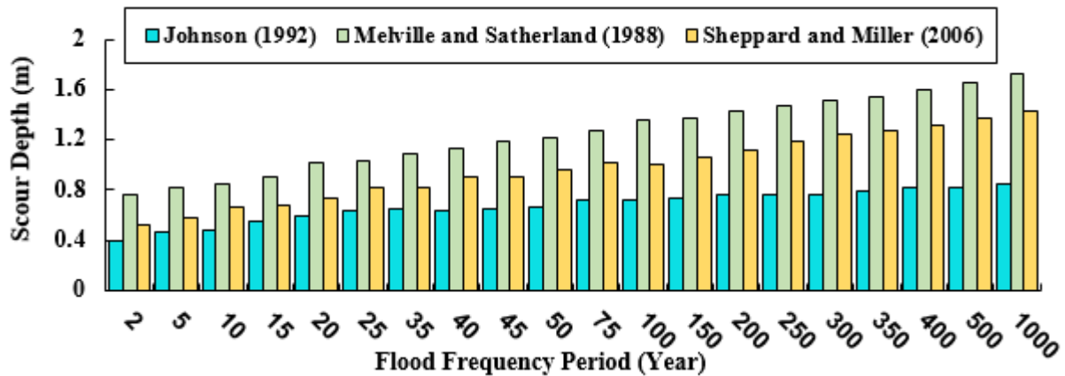
Fig. 8. The depth of Simineh Rood pier scouring using Johnson (1992), Melville and Satherland (1988) and Sheppard and Miller (2006)
