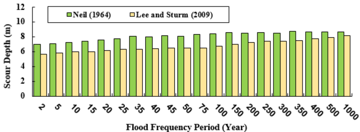
Fig. 9. Scour depth of the bridge structures of the Simineh Rood using the equations between Lee and Sturm (2009) and Neil (1964)
