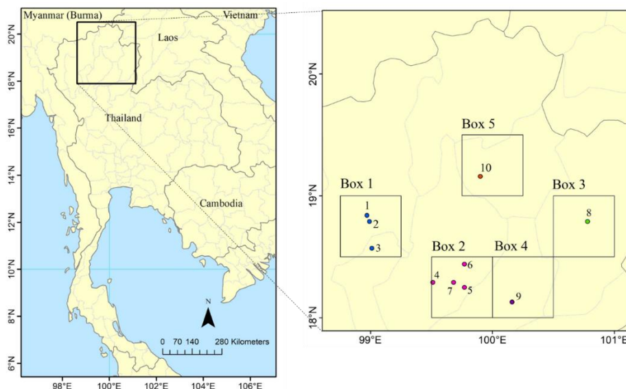
Fig. 1. Locations of 10 PCD stations and 5 satellite grid boxes.
