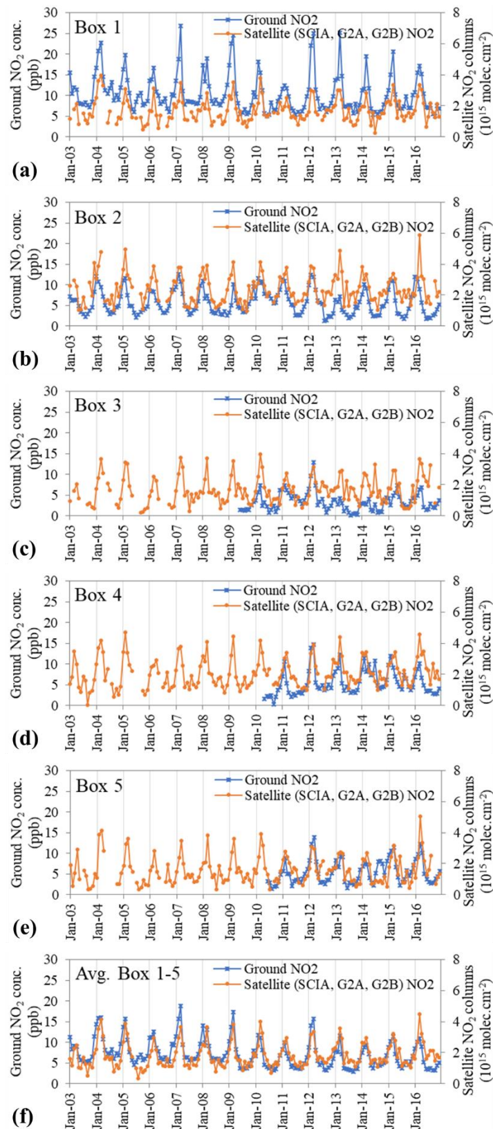
Fig. 5. Time series of morning satellite (SCIAMACHY, GOME-2A, and GOME-2B) \text{NO}_2 columns and ground \text{NO}_2 concentrations (9:00-12:00 LT) for box ID 1 (a), box ID 2 (b), box ID 3 (c), box ID 4 (d), box ID 5 (e), and all 5 boxes average (f).
