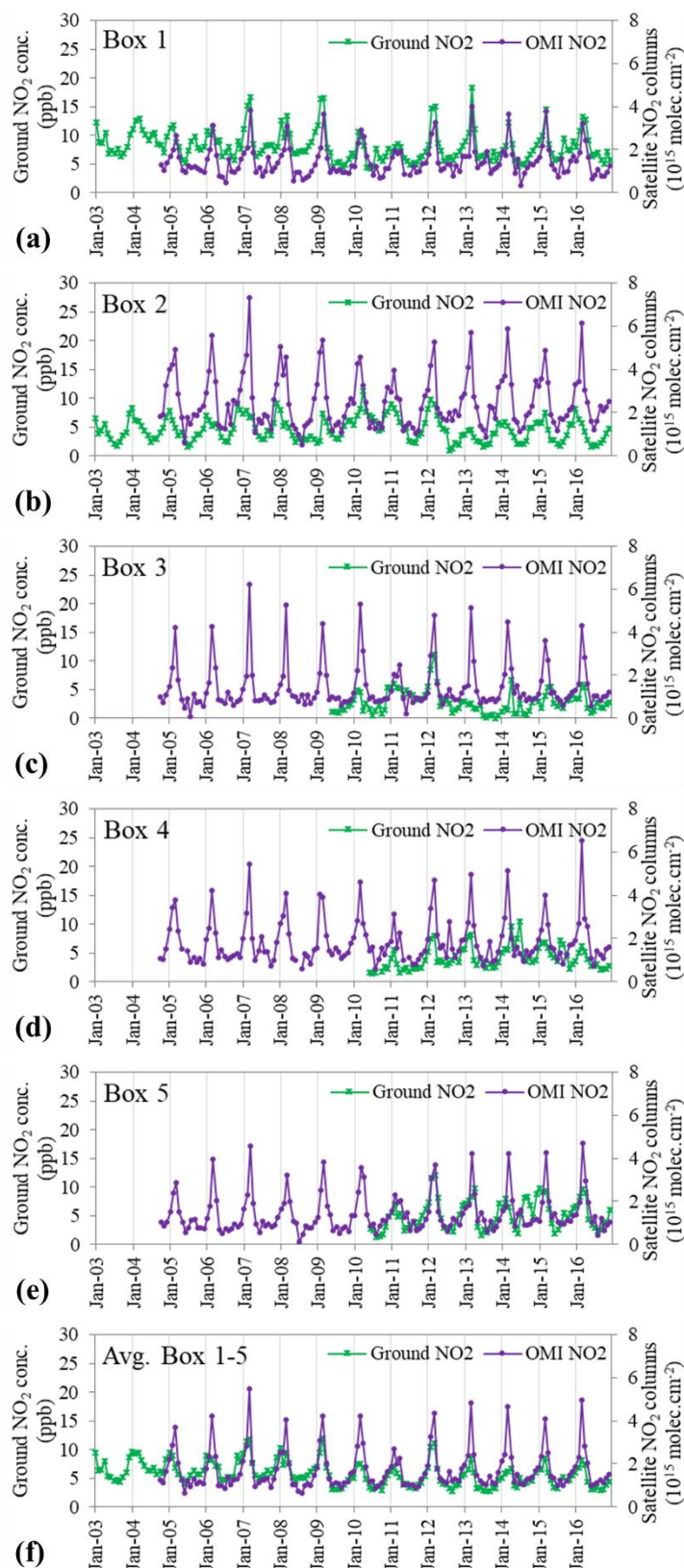
Fig. 6. Time series of afternoon satellite (OMI) NO 2 columns and ground NO 2 concentrations (12:00-15:00 LT) for box ID 1 (a), box ID 2 (b), box ID 3 (c), box ID 4 (d), box ID 5 (e), and all 5 boxes average (f).
