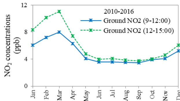
Fig. 7. Monthly mean ground NO 2 concentrations in the morning and in the afternoon.
