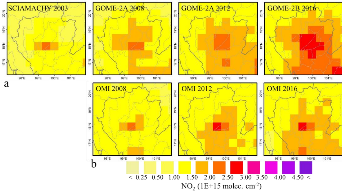
Fig. 9. Spatial distributions of annual mean tropospheric NO 2 columns from the morning satellites (a) and the afternoon satellite (b).
