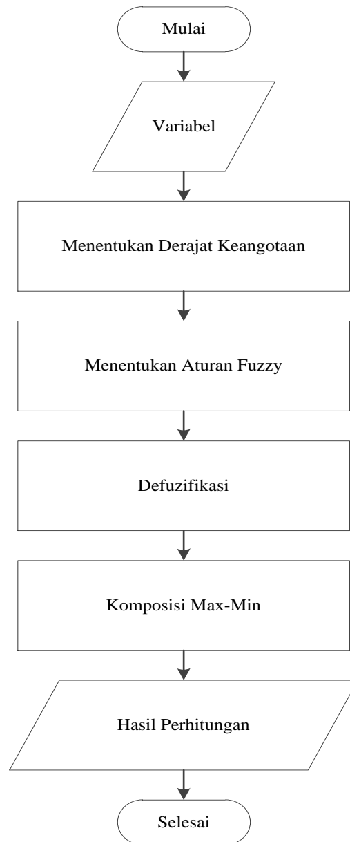
Figure 1 Flowchart Fuzzy Logic
