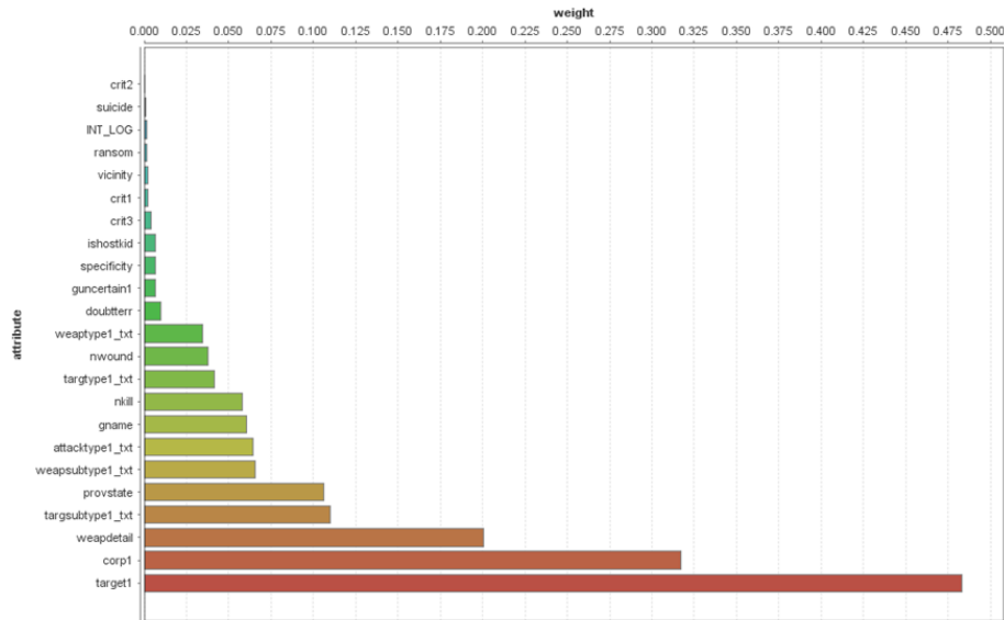
Figure 3. Feature Importance
