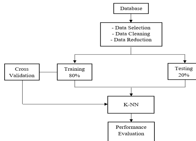
Figure 1. Research Design
