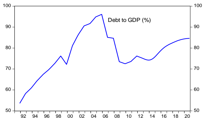
Figure 4. The forecasted value of public debt to GDP ratios for scenario (1)
