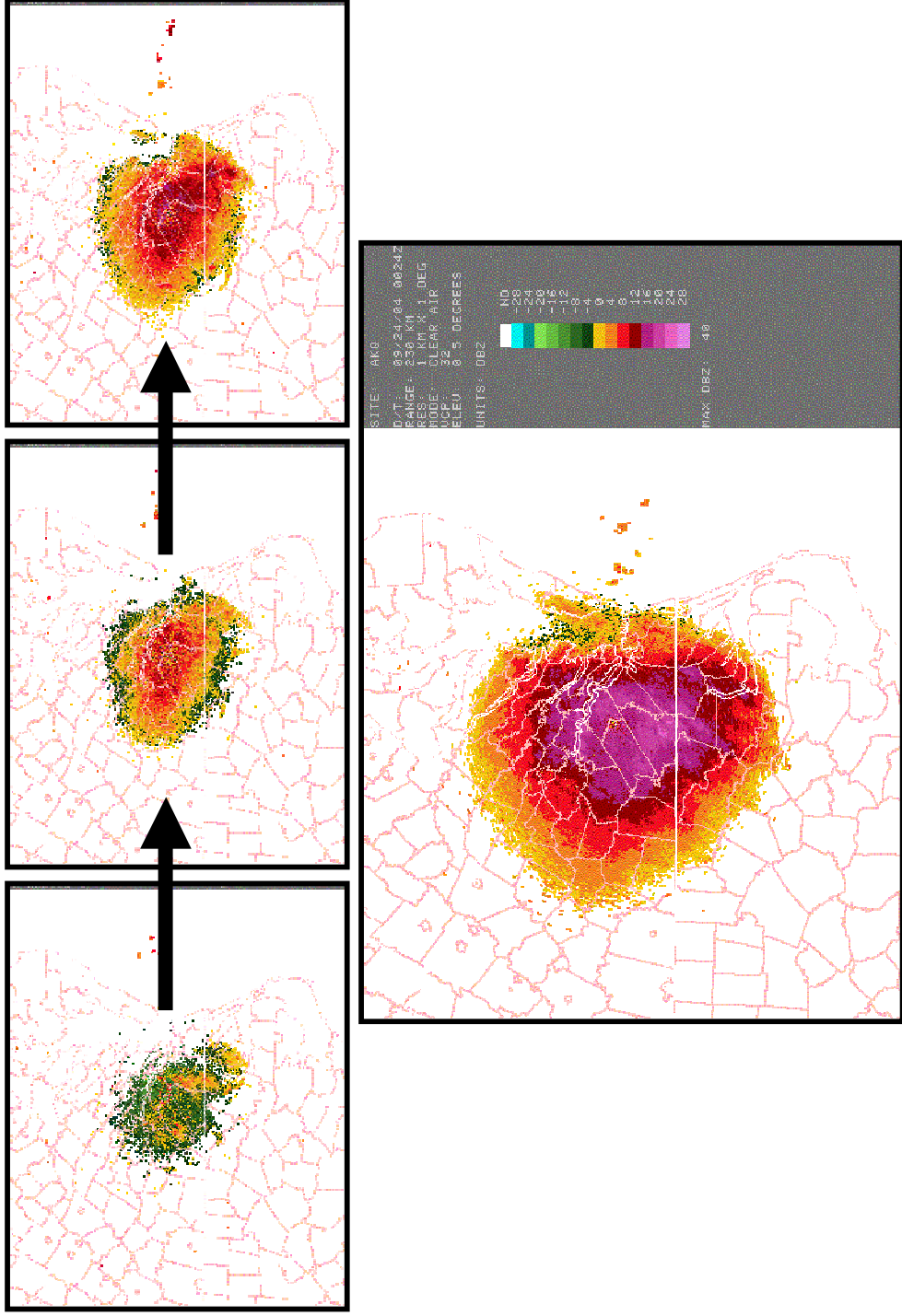
Figure 1. Figure 2. Temporal progression of migrants emerging from the landscape as recorded by the Wakefield, VA NEXRAD. Initial image from a scan approximately 15 min after sunset; next two images taken after successive 20 min intervals. The last image taken 40 min after the third (approximately 1.5 hr after sunset). The final image depicts “saturation” of the radar’s ability to detect further increases in numbers of biological targets in the atmosphere.
