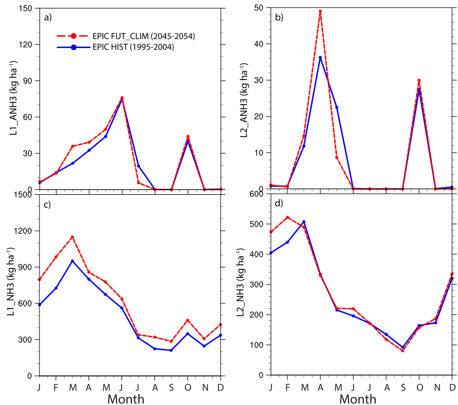
Figure 4. Ten-year average monthly values of HIST (blue) and FUT_CLIM (red) CBA area-totaled NH 3 (a–b) fertilizer application rate (L1_ANH3 and L2_ANH3) and (c–d) layer content (L1_NH3 and L2_NH3) for the sum (rainfed + irrigated) of all 2006 NLCD-BELD4 crop types.
