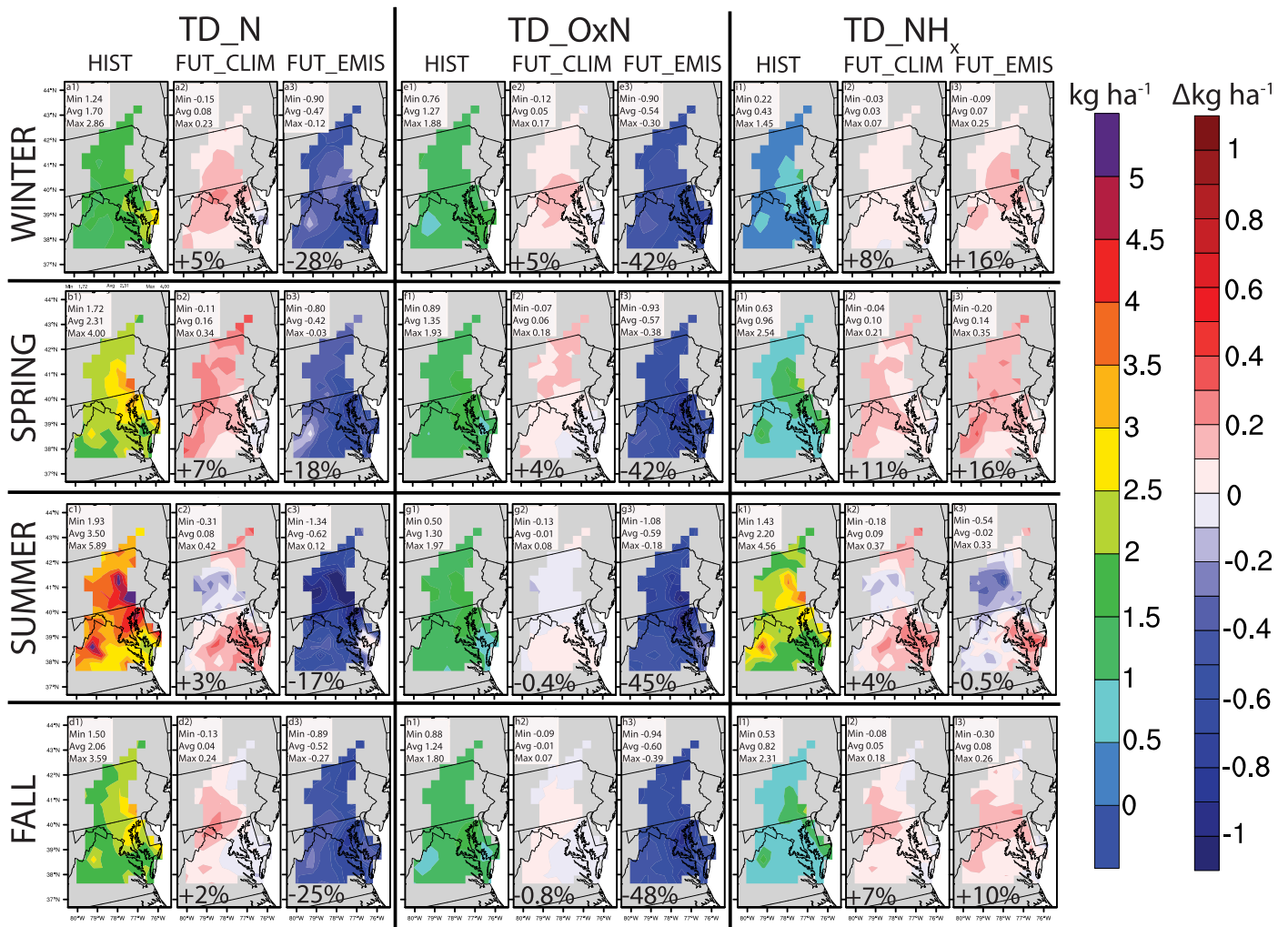
Figure 5. Spatial plots of the 10-year average seasonal totals (HIST; column 1) and absolute differences (FUT_CLIM, column 2, and FUT_EMIS, column 3) for (a–d) TD N , (e–h) TD O x N , and (i–l) TD NH x in the CBW. The average relative changes (defined in Table 1) are shown in the bottom left-hand corner of each FUT_CLIM and FUT_EMIS panel (based on Figure S22).
