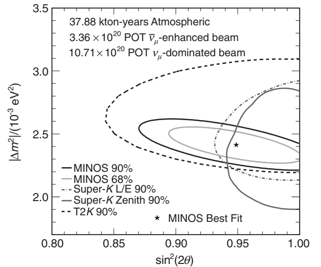
FIG. 2. The allowed regions of |\Delta m^2| and \sin^2(2\theta) , assuming identical neutrino and antineutrino oscillations. The MINOS result is compared to results from the Super-Kamiokande [25] and T2K [26] Collaborations.
