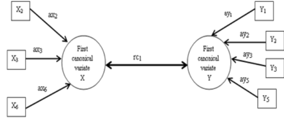
x_2 Variable in X data set y_1 Variable in y data set ax_2 Loading of correlation with ith x variable on canonical variate x ay_1 Loading of correlation with ith y variable on canonical variate y rc_1 Canonical correlation for the first pair of canonical variates
