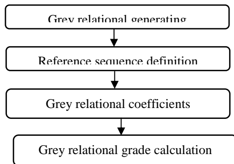
Fig. 2: Procedure of the grey relational analysis (Kuo et al. ) The likeness between the dependent feature and the independent feature are the most determining, especially when FGRA is used in the case of selecting the most predictive features. The features that have high similarity will set up the optimal feature set. The FGRA is also used to retrieve the nearest projects to the reference project by measuring the similarity degree between the reference project and all other comparative projects.
