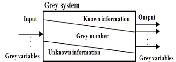
Fig.1: The concept of a grey system (Lee et al.)
