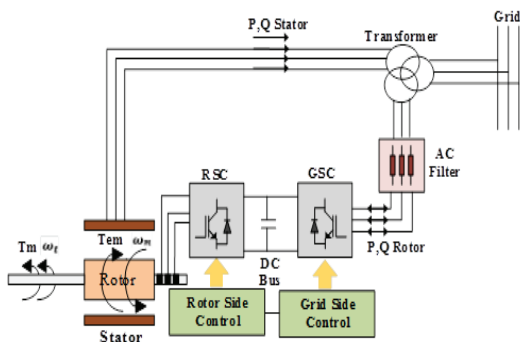
Fig. 1. Schematic representation of a DFIG-WT setup
