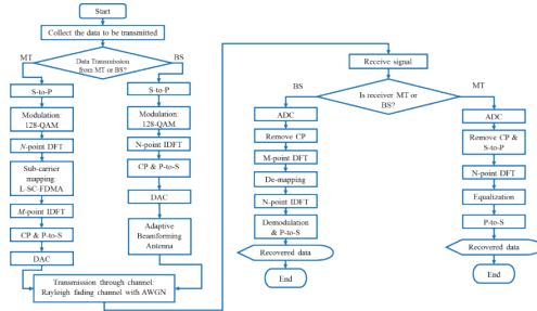
Fig. 1. Designed mm-wave network's architectural flow chart
