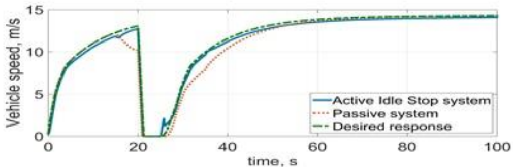
(c) Vehicle speed against time at 25 degree road gradient
