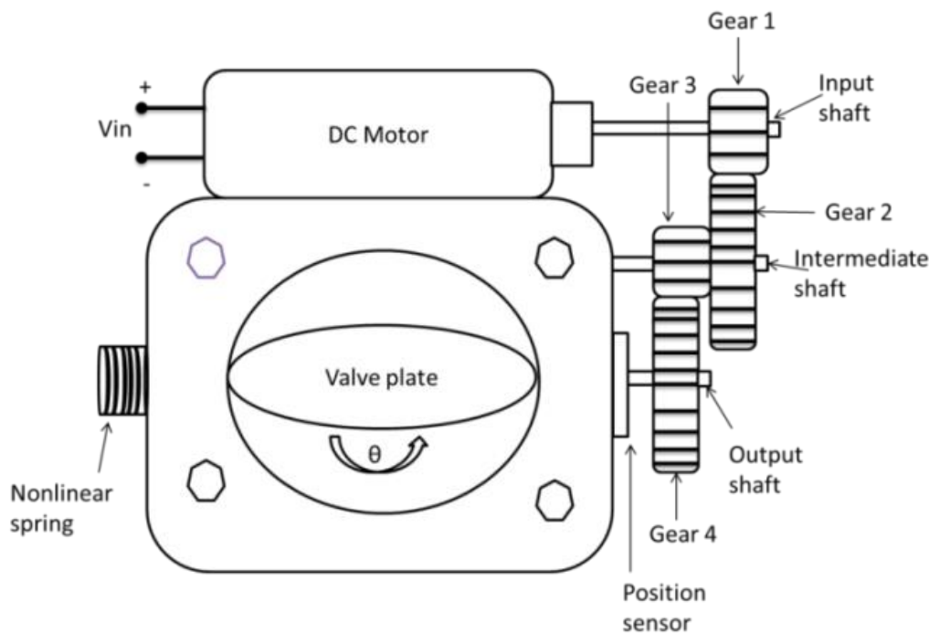
Figure 5. Electronic throttle body
