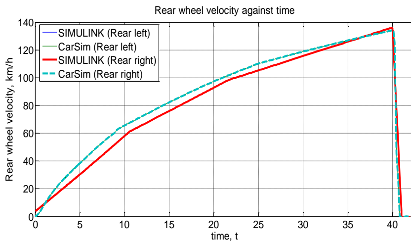
(c) Rear wheel velocity against time
