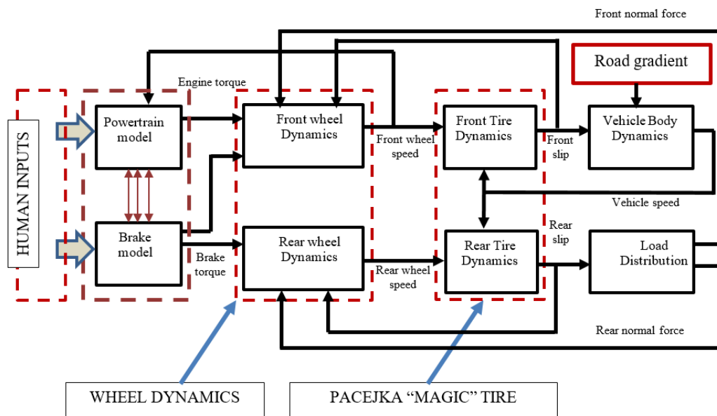
Figure 1. Vehicle Longitudinal Model Block Diagram
