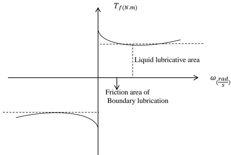
Figure 6. Frictional effect
