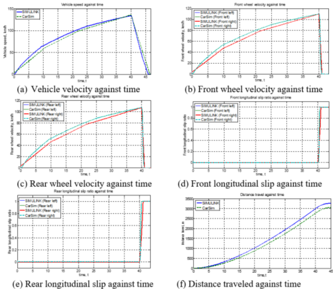
Figure 3. Vehicle response at throttle input of 50% and sudden braking
