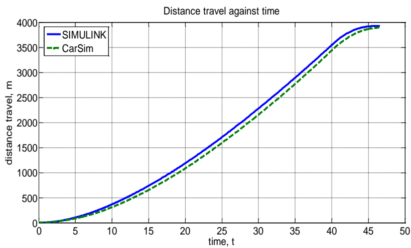
(f) Distance traveled against time
