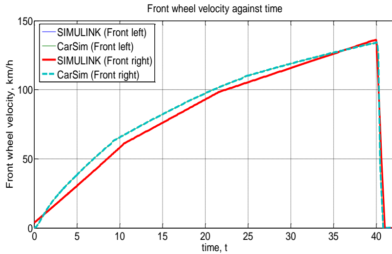
(b) Front wheel velocity against time
