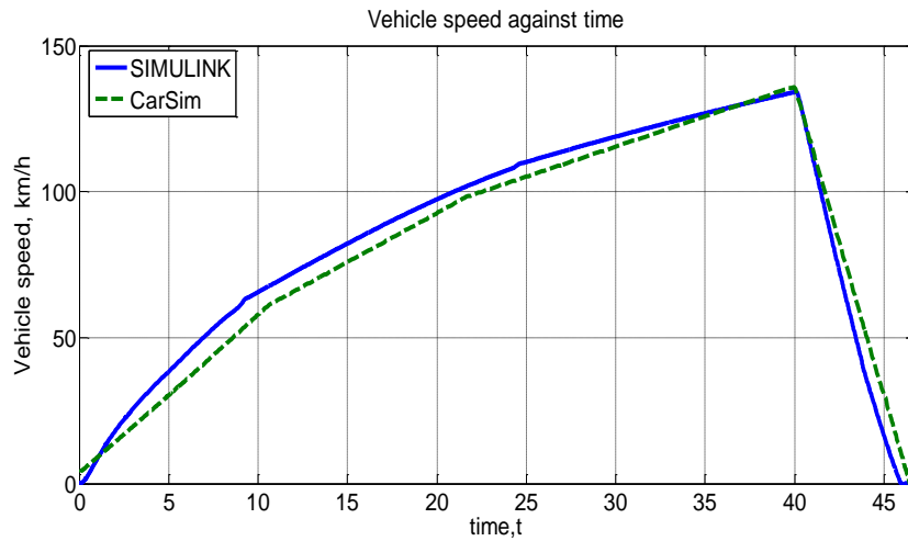
(a) Vehicle velocity against time
