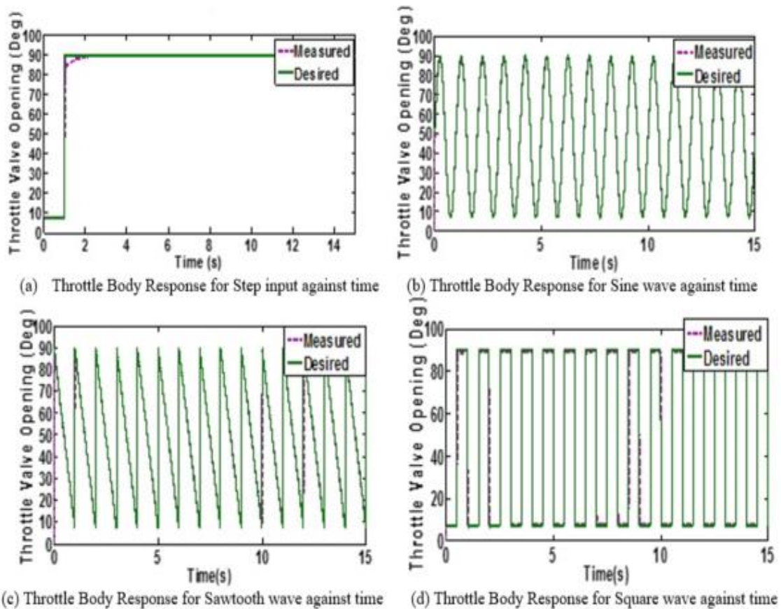
Figure 9. Position tracking response of the inner loop model using electronic throttle body
