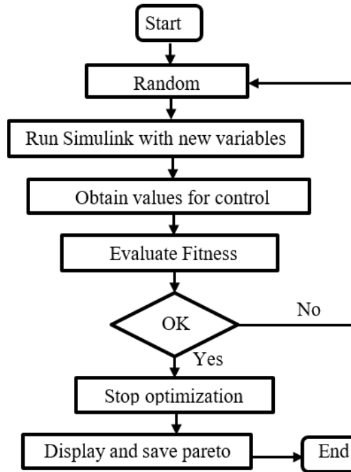
Figure 11. Flowchart of optimization process using a genetic algorithm
