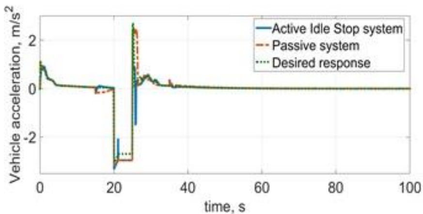
(c) Vehicle acceleration against time at 25 degree road gradient
