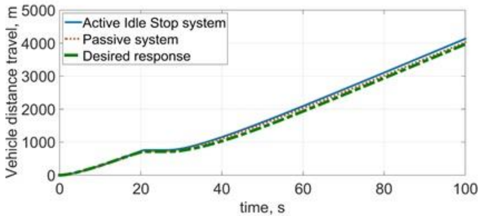
(b) Vehicle distance travel against time at 20 degree road gradient
