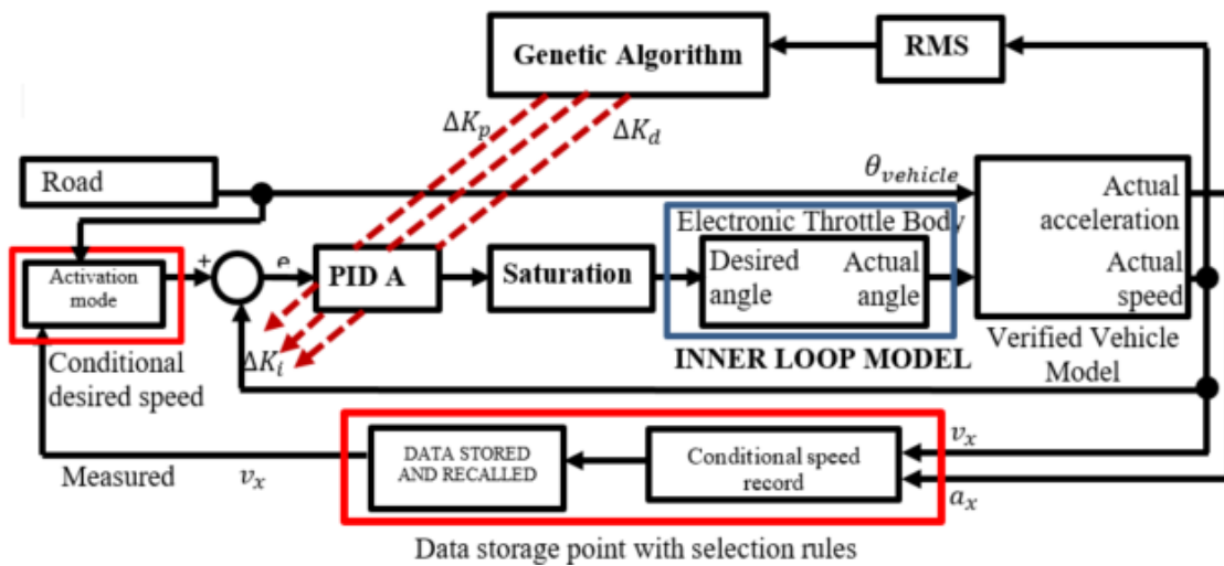
Figure 10. AIS system control structure
