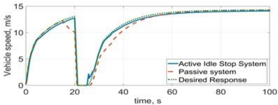
(a) Vehicle speed against time at 15 degree road gradient
