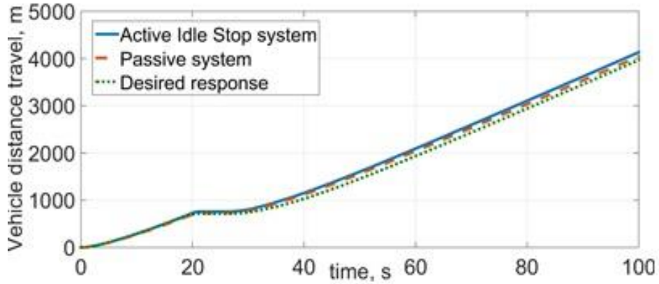
(a) Vehicle distance travel against time at 15 degree road gradient
