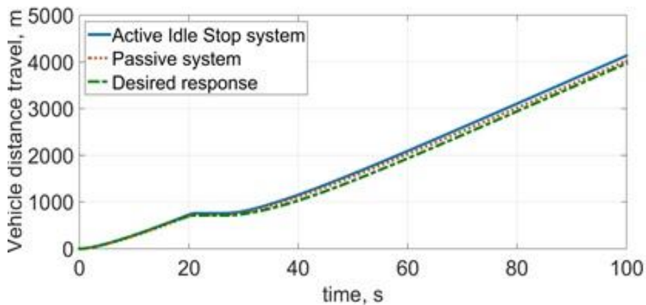
(c) Vehicle distance travel against time at 25 degree road gradient
