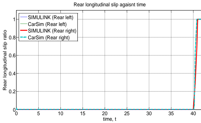
(e) Rear longitudinal slip against time
