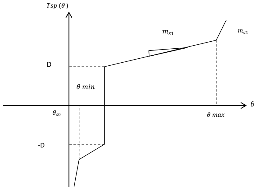
Figure 7. Nonlinear spring
