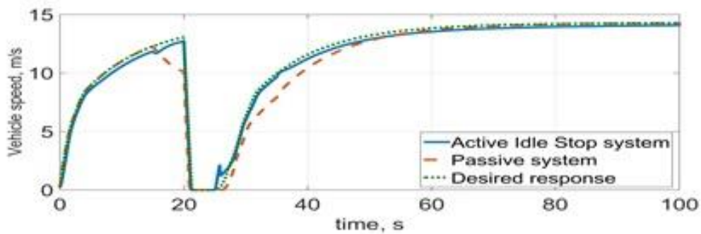
(b) Vehicle speed against time at 20 degree road gradient
