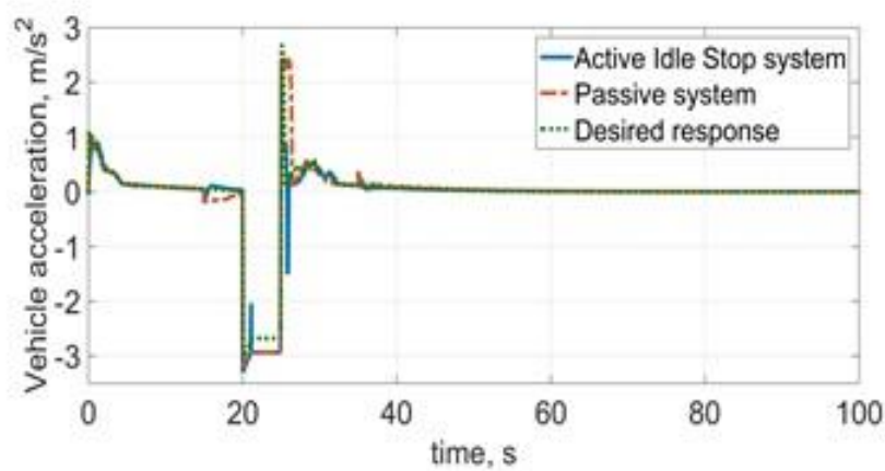
(b) Vehicle acceleration against time at 20 degree road gradient
