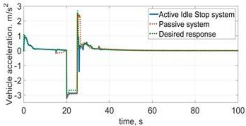
(a) Vehicle acceleration against time at 15 degree road gradient
