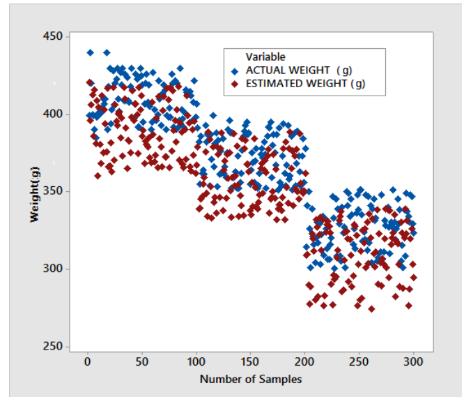
Figure 12: Scatter plot of actual weight and estimated weight versus the number of Harumanis mango samples
