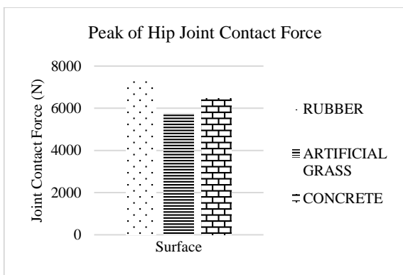
Figure 6: Peak contact force at the hip joint
