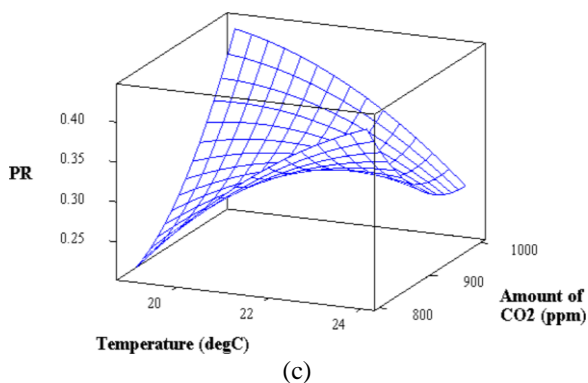
Figure 6: Plot showing (a) interaction of light intensity and temperature and its effect on photosynthetic rate, (b) interaction of light intensity and amount of CO 2 and its effect on photosynthetic rate, and (c) interaction of temperature and amount of CO 2 and its effect on photosynthetic rate.
