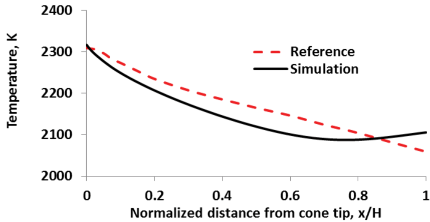
Figure 4: Simulation temperature distribution compared with the reference temperature distribution [13-15].
