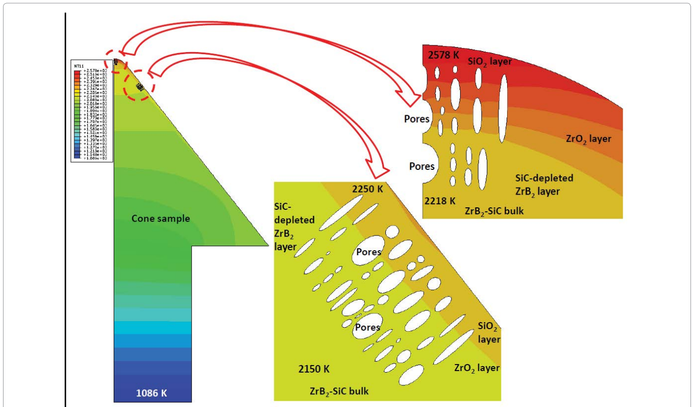
Figure 7: Distribution of temperature in the inner body of the cone.
