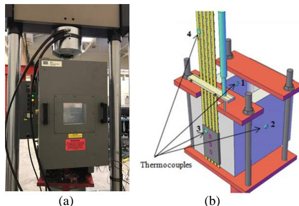
Fig. 2. Test setup (a) heating and cooling chamber, (b) locations of thermocouples.
