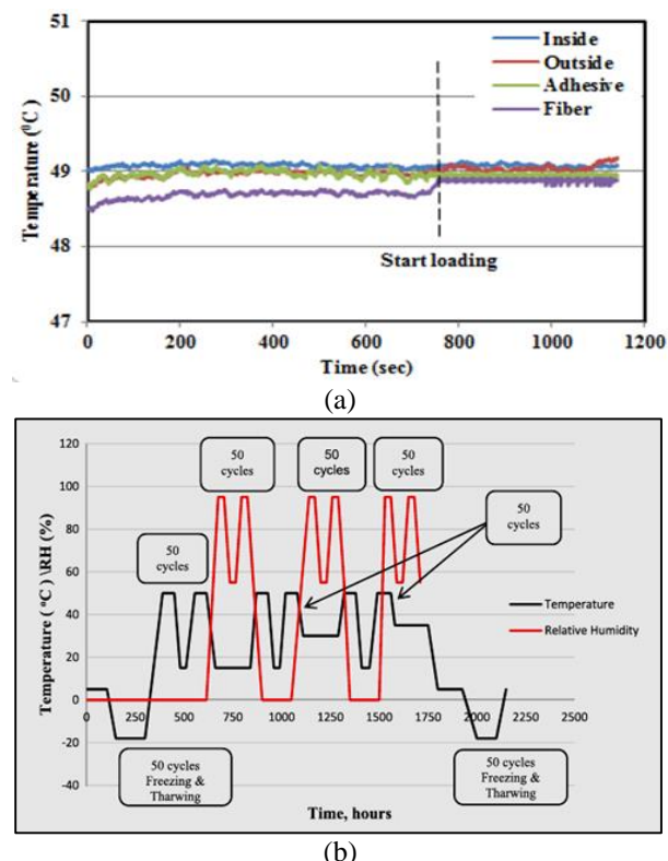
Fig. 3. Applied temperature (a) Time-temperature curve obtained from the four thermocouples, (b) cycles of temperature exposure regime.
