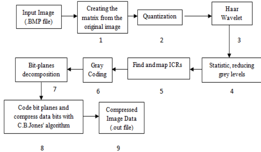
Figure 3. The Scheme of lossy image compression with DHWT and ICRs
