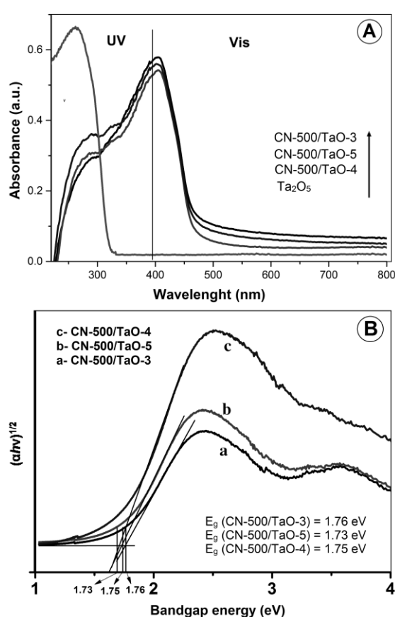
Figure 3: (A) UV-Vis DRS and (B) band gap energy of Ta 2 O 5 , CN-500/TaO-3, CN-500/TaO-4, CN-500/TaO-5
