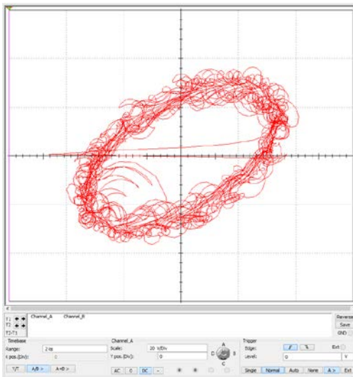
c) Plano YZ
