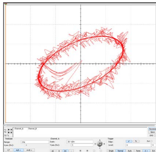
d) Plano XZ
