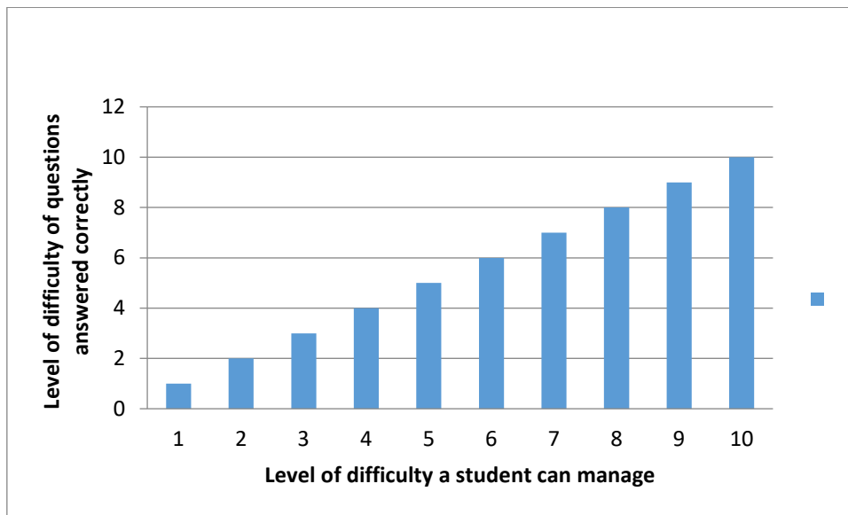
Figure 1: Perfect implicationality of difficulty
