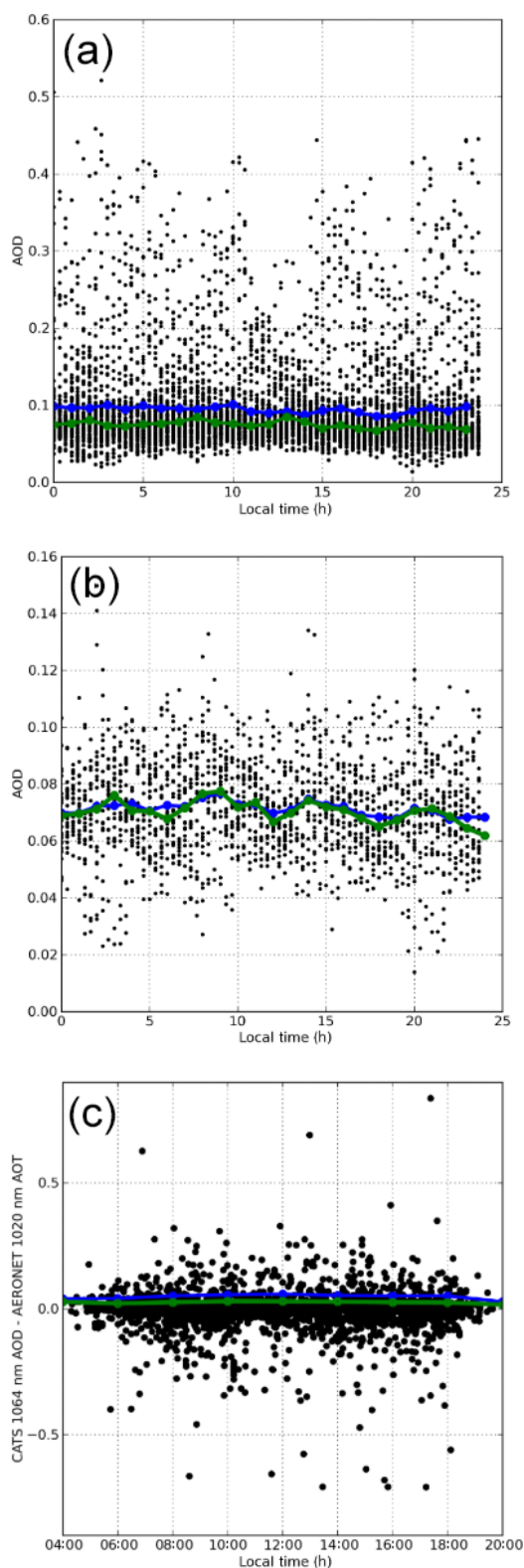
Figure 4. CATS 1064 nm AOD (a) as a function of local time for the globe and (b) as a function of local time for areas south of -25^{\circ} . The difference between CATS 1064 nm AOD and AERONET 1020 nm AOD as a function of local time is shown in panel (c). The mean is represented by the blue line, while the median is the green line.
