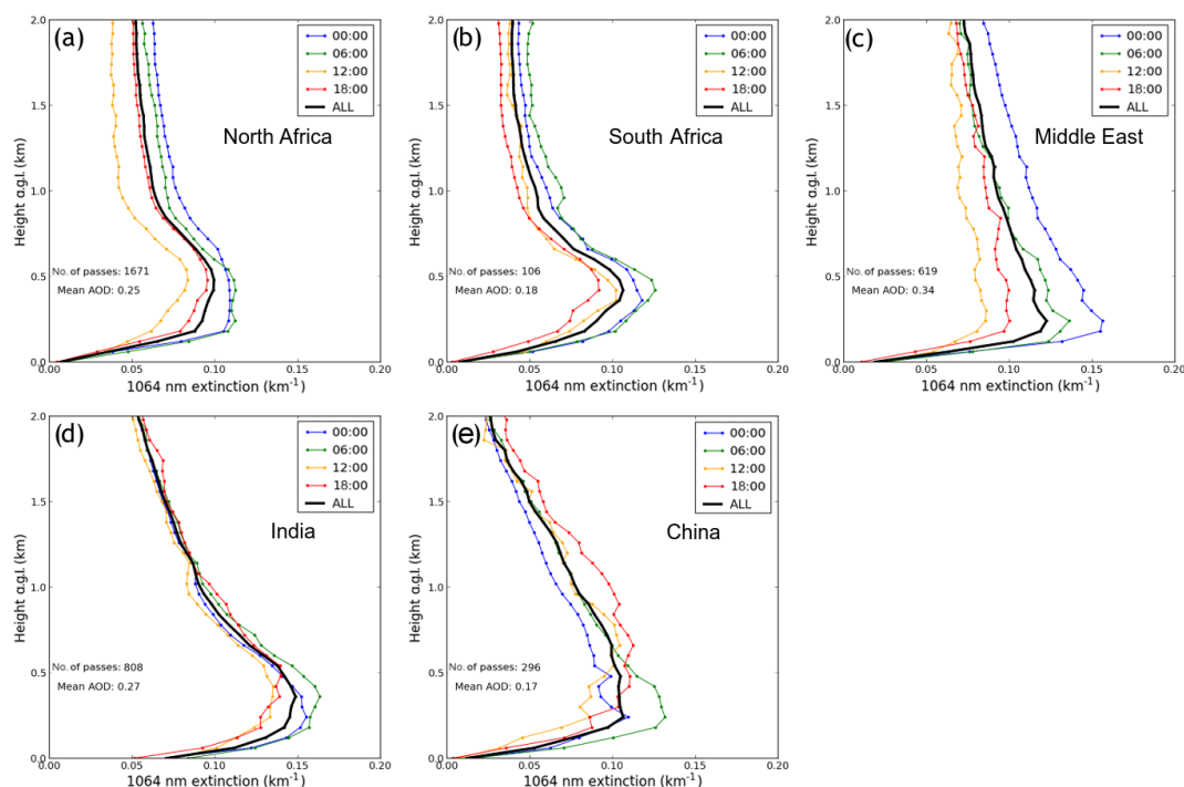
Figure 13. JJASON 6 h average (00:00, 06:00, 12:00 and 18:00 LT) vertical profiles of CATS 1064 nm for locations shown in Fig. 6b; (a) north Africa, (b) south Africa, (c) the Middle East, (d) India and (e) northeast China.
