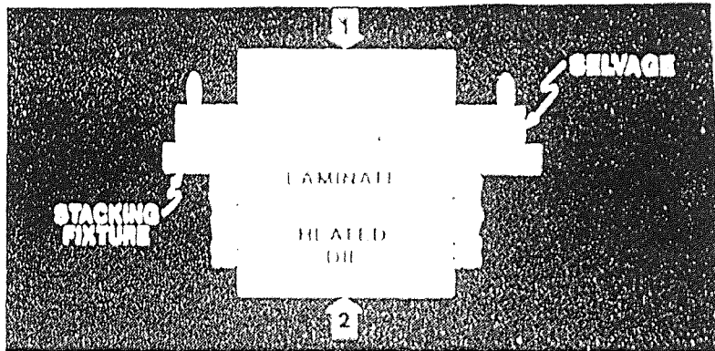
Figure 2.5. Lamination
