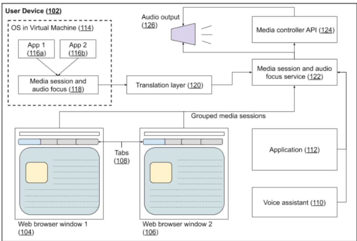
Fig. 1: Audio output determined by unified management of media sessions and audio focus
