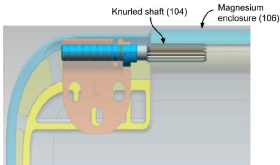
Fig. 1: A knurled shaft used in conjunction with a magnesium alloy enclosure
