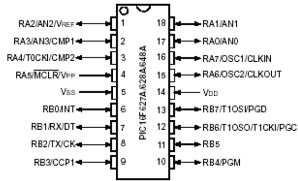
Figura 2: Layout PIC 16F628A
