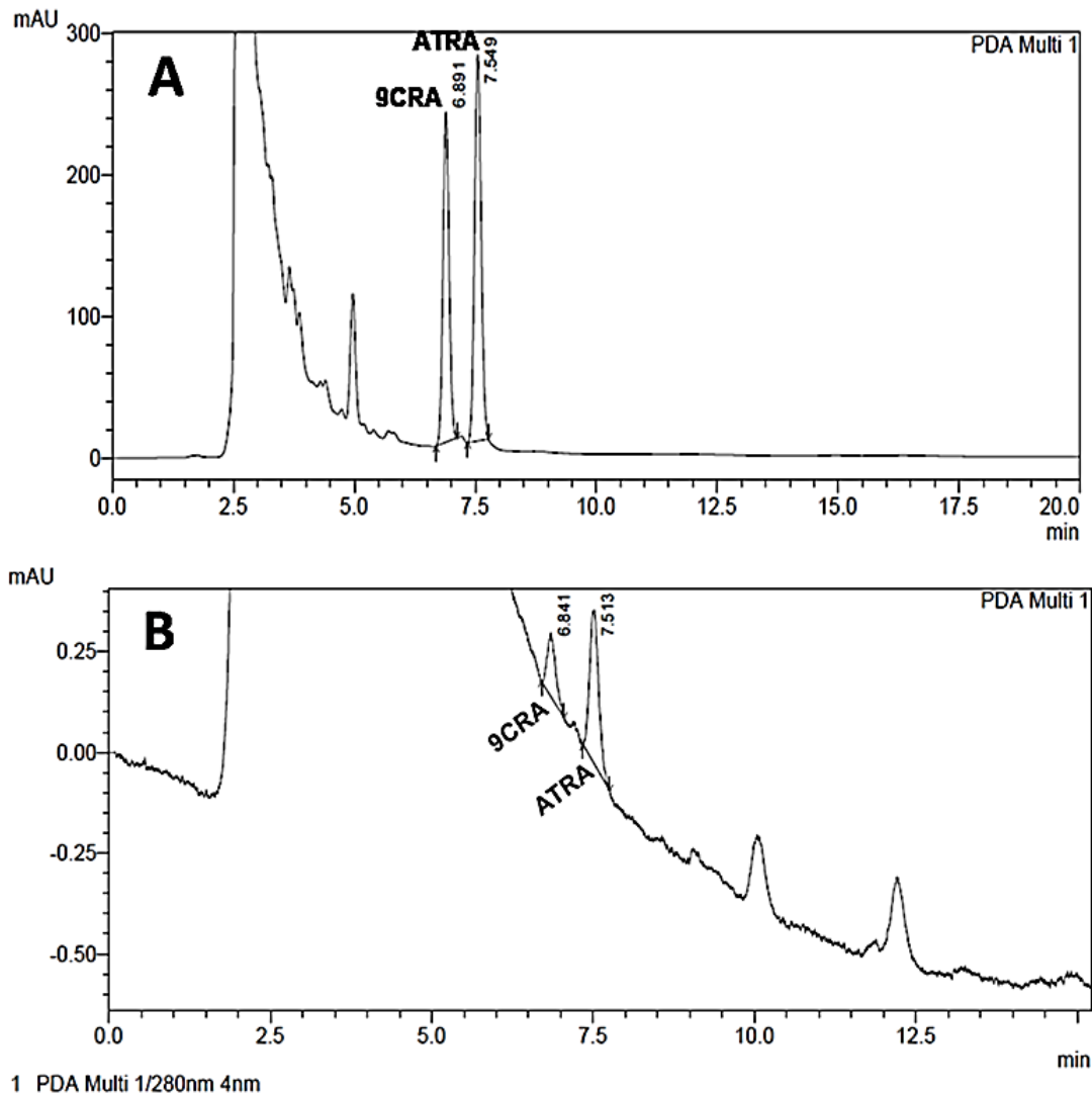
Figure 1. HPLC chromatogram of retinoic acid isomers (ATRA: all-trans retinoic acid; 9CRA: 9-cis retinoic acid); A: standard mixture B: analysis in mature ovaries of mud crabs, Scylla serrata .
