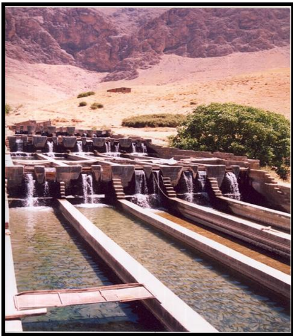
Figure 2. Raceways used for aquaculture in the area of Sarab Gerdu, Iran.
