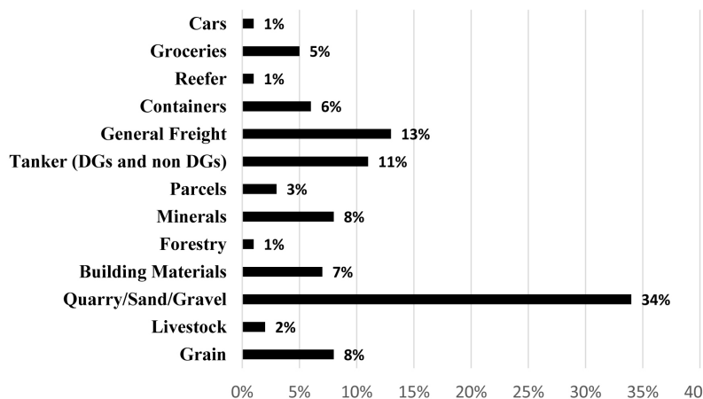
Fig. F2. Commodities carried profile carried by PBS Vehicles. Survey 2 2013-2016.
