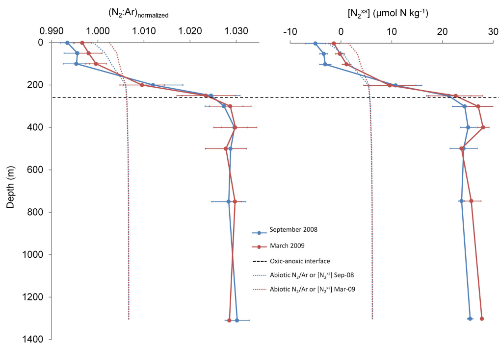
Fig. 5. Profiles of normalized N_2/Ar ratios and [N_2^{X_S}] in the Cariaco Basin during September 2008 and March 2009. Background (abiotic) N_2/Ar ratios and [N_2^{X_S}] were estimated using data collected at BATS (see Sect. 3.2).
