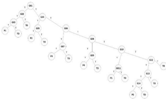
Gambar 1 decision tree
