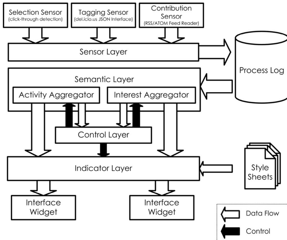
Fig. 3. Component interaction of the prototype
