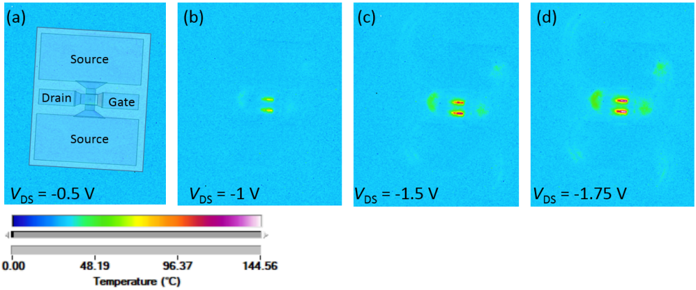
Figure 4.8: Infrared images of a GFET on 1\ \mu\text{m}/300\ \mu\text{m} \text{SiO}_2/\text{Si} substrate with gate length L_g = 0.5\ \mu\text{m} and gate width W_g = 2 \times 15\ \mu\text{m} at the same gate-source bias V_{GS} = 1.5\ \text{V} and different drain-source biases of (a) V_{DS} = -0.5\ \text{V} , (b) V_{DS} = -1\ \text{V} , (c) V_{DS} = -1.5\ \text{V} , and (d) V_{DS} = -1.75\ \text{V} . A QFI InfraScope is used to visualize the heating of the GFET. In the IR microscope setup the dual-channel Keithley Source Meter 2604B is used for biasing.
