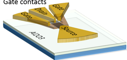
Figure 3.3: Fabrication process of the GFET in PAPER G. In contrast to the fabrication process of the GFETs in Fig. 3.2, the gate was formed first. This way the graphene is accessible for the near-field terahertz nanoscopy.
