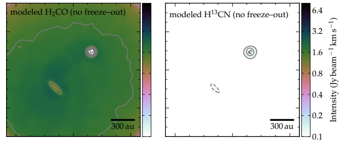
Fig. C.1. Radiative transfer model maps (see Sect. 4.1) of \text{o-H}_2\text{CO} 5 1,5 –4 1,4 ( left ) and \text{H}^{13}\text{CN} 4–3 ( right ) with freeze-out effects ignored. These maps are counterparts of the more physically correct ones where freeze-out is implemented, in the middle right and bottom right panels of Fig. 6. Color scales and contours are identical to those used in Fig. 6, with the exception that negative intensity contours (dashed) are included in this figure.
