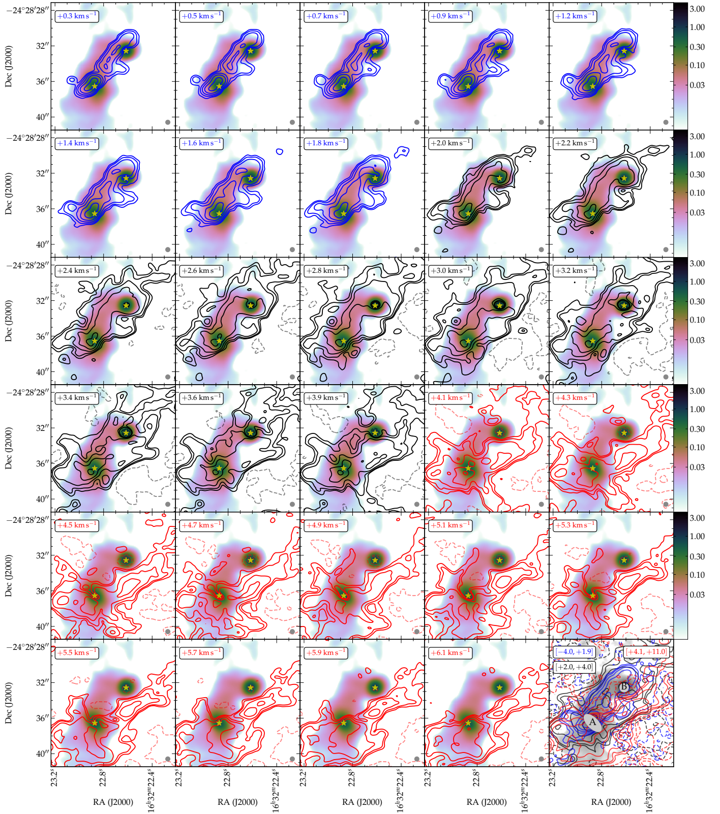
Fig. B.3. \text{H}_2\text{CO } 5_{1,5}-4_{1,4} channel maps. As Fig. B.1. First positive (negative) contour level in individual channel maps: 0.12 ( -0.24 ) \text{Jy beam}^{-1} ; first contour levels in the bottom right integrated ranges panel: 0.2 \text{ Jy beam}^{-1} \text{ km s}^{-1} .
