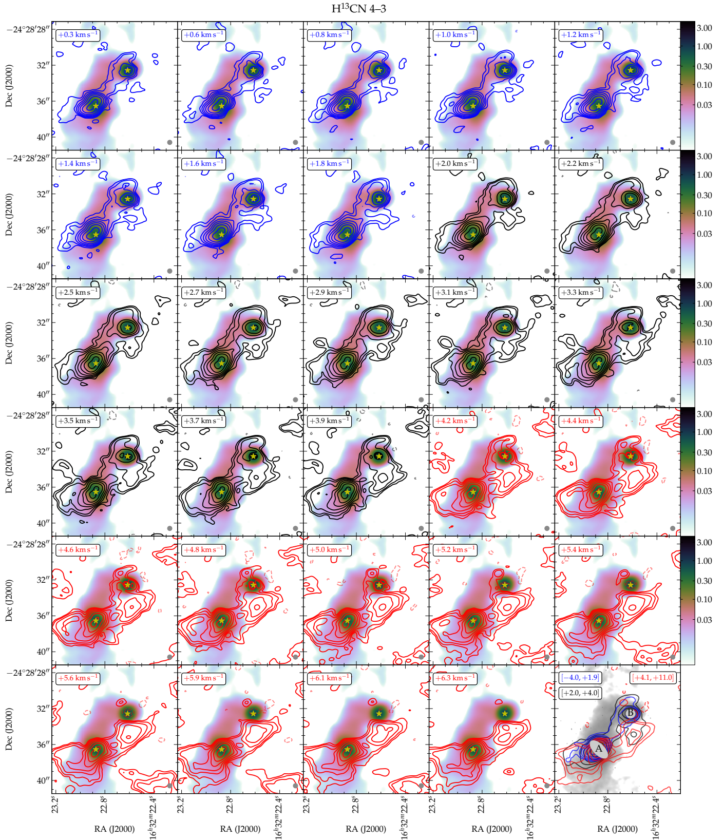
Fig. B.2. \text{H}^{13}\text{CN} 4-3 channel maps. As Fig. B.1. First positive (negative) contour level in individual channel maps: 0.03 ( -0.06 ) \text{Jy beam}^{-1} ; first contour levels in the bottom right integrated ranges panel: 0.2 \text{Jy beam}^{-1} \text{ km}^{-1} .
