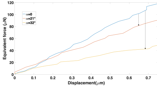
Figure 4.14: Effect of FMS tilt on measured force values.
