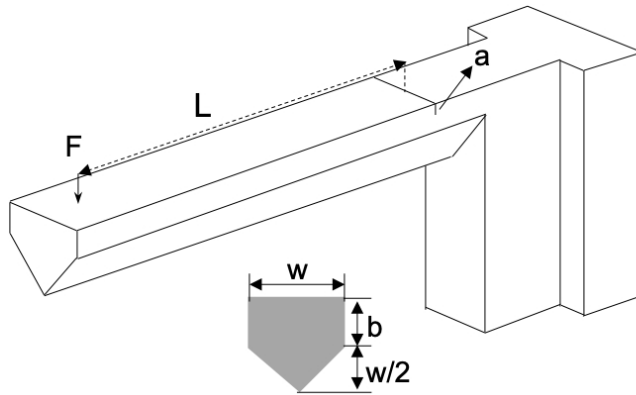
Figure 4.19: Schematic of pentagonal cross section cantilevers with FIB milled notch.
