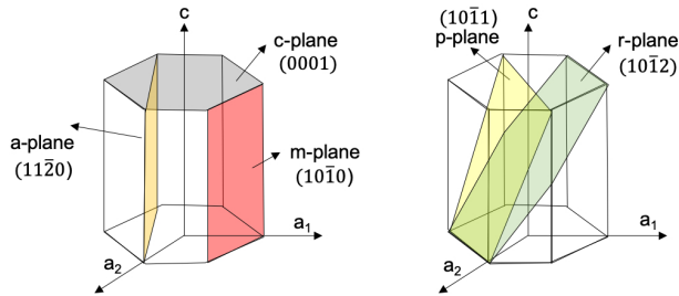
Figure 2.2: Schematic of hcp unit cell showing different crystallographic planes.
