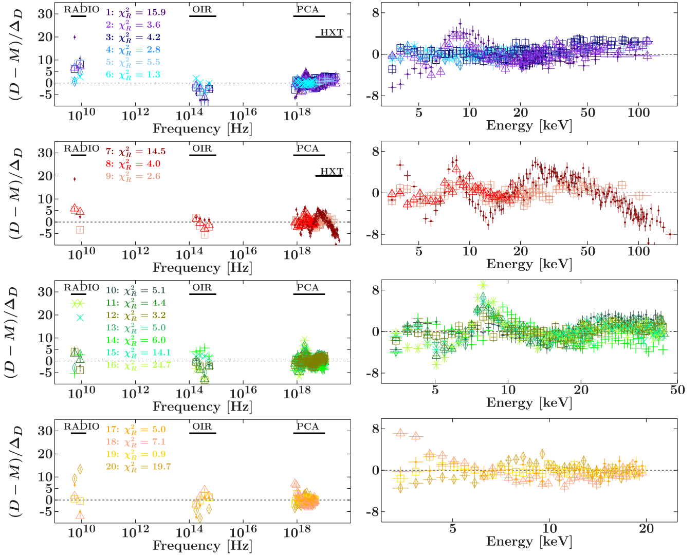
Figure 9. Standardized residuals [(data-model)/uncertainty] of fits to all 20 broad-band spectra of GX 339–4 with Model B1 (jet IC-dominated X-ray spectra): t\text{babs} \times [\text{reflect}(\text{agnjet}) + \text{Gaussian}] , with typical \chi_R^2 \sim a few to 10 s. Each panel shows fits to observations within 2005, 2007, 2010, and 2011, respectively. Radio, OIR, and X-ray data are labelled, and different symbols/colours indicate the broad-band data-model residuals for each fit. The X-ray spectra are dominated by jet SSC and IC scattering of disc photons in the jet, as well as reflection off the disc.
