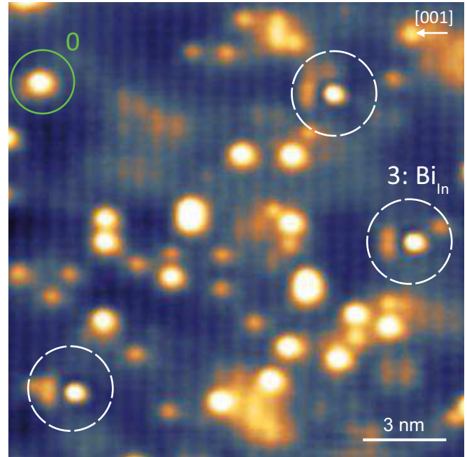
FIG. 7. High-resolution filled state X-STM image with potential \text{Bi}_{\text{In}} antisites [class (3)] with a valence of 5 in the surface layer next to commonly observed isovalent \text{Bi}_{\text{P}} substitutional atoms. An isovalent \text{Bi}_{\text{P}} atom in the cleavage plane [class (0)] is marked for comparison. The image is taken on F2 in sample B at I_T = 40 pA and V_{\text{bias}} = -2.5 V. The growth direction is indicated by an arrow.
