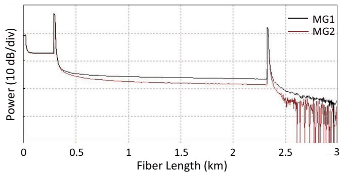
Fig. 4. Measured OTDR curves of both MGs.
