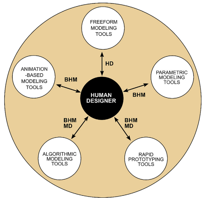
Fig. 3. Modes of human-machine interactions featured in the hybrid platform (HD = human-dominated mode; MD = machine-dominated mode; BHM = balanced human-machine mode).
