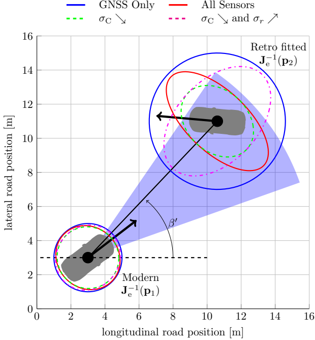
Figure 1. Illustration of 1-sigma ellipses representing the CRLBs \mathbf{J}_e^{-1}(\mathbf{p}_1) and \mathbf{J}_e^{-1}(\mathbf{p}_2) for a two vehicle scenario with a modern vehicle with position \mathbf{p}_1 and a retrofitted vehicle with position \mathbf{p}_2 . First we see the uncertainty in the positions given that we only take into account the GNSS measurements (solid blue). Then we see how the uncertainty changes when incorporating the radar ( \sigma_\alpha = 0.3 and \sigma_r = 0.12 ) as well as the compass ( \sigma_C = 1 ) from the modern vehicle (solid red). We also see how the uncertainty about the retrofitted vehicle decreases in the direction \beta' + \pi/2 when decreasing the uncertainty in the modern vehicles compass to \sigma_C = 0.2^\circ (dashed green), and how the uncertainty about the retrofitted vehicle is increased in the direction \beta' if we in addition increase the range uncertainty of the radar to \sigma_r = 12 (dashed magenta). Note that parameter values used here might differ from Section V.
