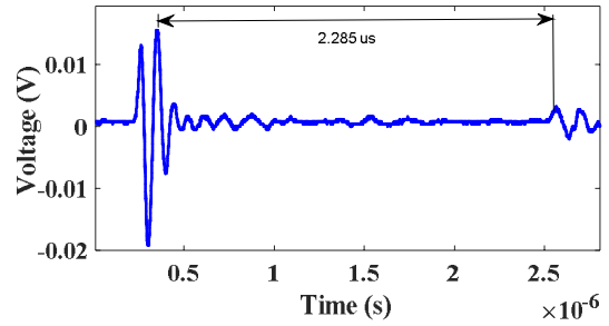
FIGURE 9. Original and reflected pulses injected with PD calibrator in the tested cable.
