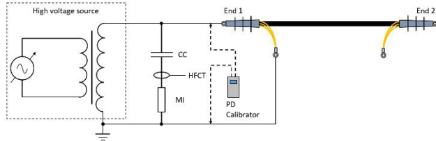
FIGURE 8. Laboratory test setup for online measurement of PDs in the MV cable (electrical layout); CC- coupling capacitor; MI- measuring impedance of commercial system.
